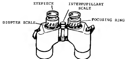
Figure 2-26. M19 binoculars.
